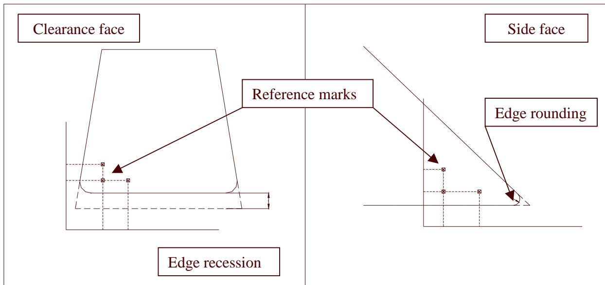
Figure 5 - The reference marks on the tooth faces, for measuring dulling and recession of the cutting edge
