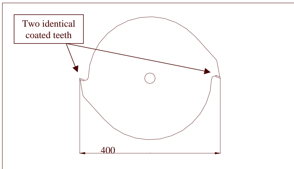
Figure 6 - The two-teeth blade type used in the tests
