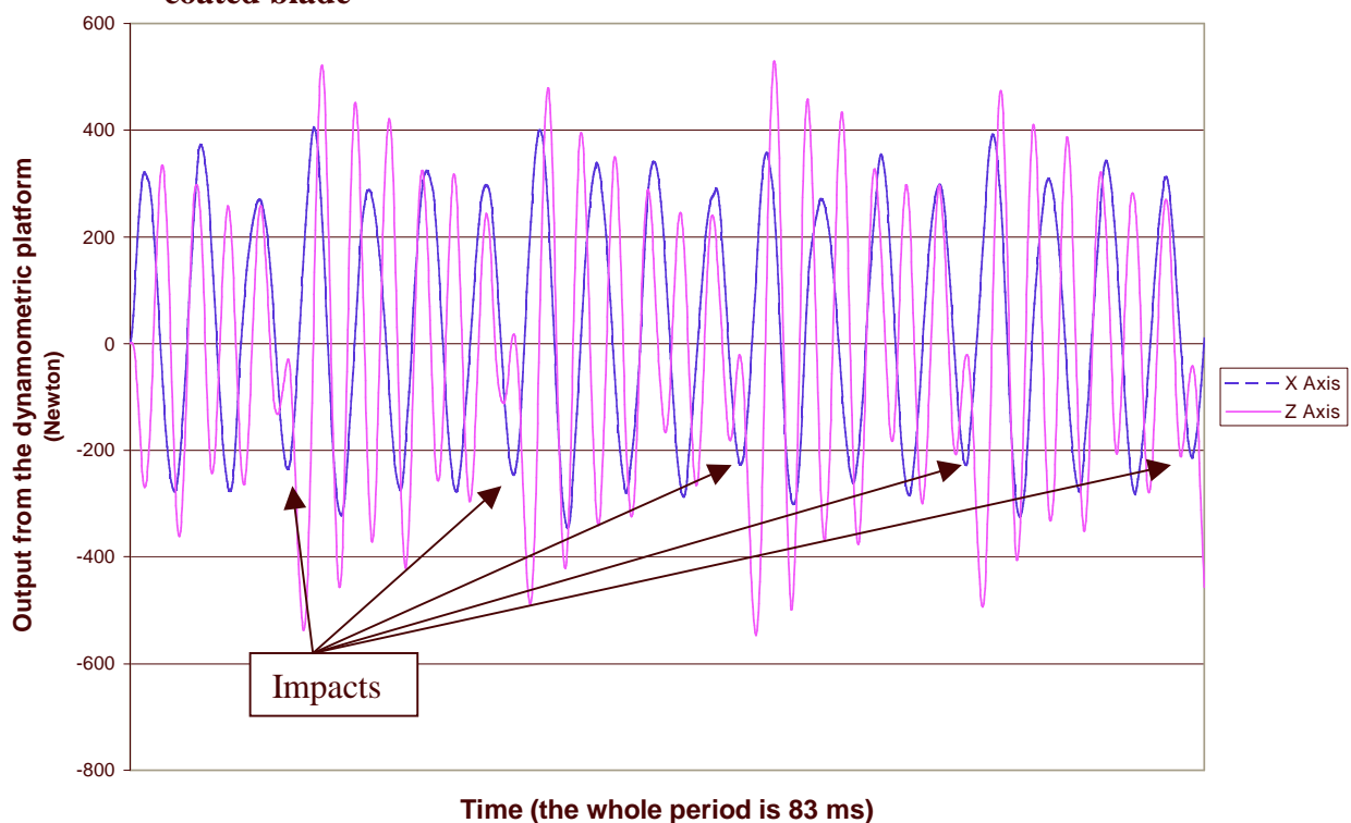
Figure 7 - Sawing test obtained processing a 60 mm thick Azobè board with a stellite coated blade
