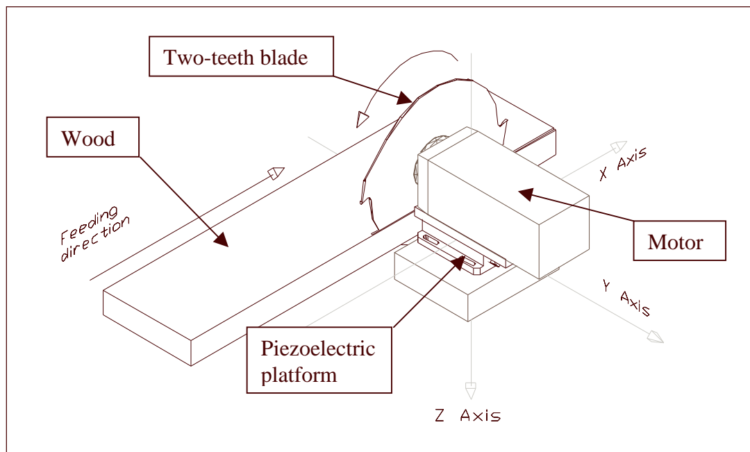
Figure 3 - Measuring system and directions of axes
