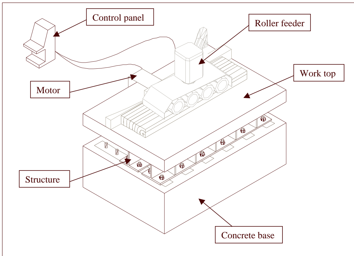
Figure 2 - The test bench
