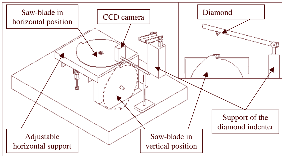
Figure 4 - The marking and measuring bench
