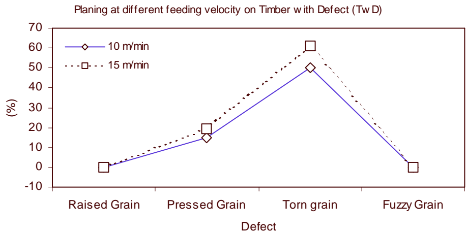
Figure 4 - Planing process performed through carbide tipped knives on a helicoidal cutter head at different feeding velocities on Timber with Defects. On the Y axis the incidence (%) of the various defects from fair to very poor quality (grade from 3 to 5) is reported
