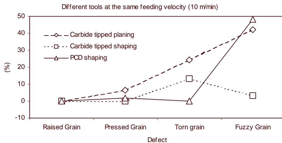
Figure 5 - Planing and shaping processes performed respectively with carbide tipped knives on a helicoidal cutter head and with moulding tools (both carbide tipped and PCD) at the same feeding velocity on Defect-Free Timber. On the Y axis the incidence (%) of the various defects from fair to very poor quality (grade from 3 to 5) is reported
