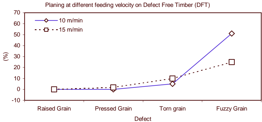
Figure 3 - Planing process performed by using carbide tipped knives on a helicoidal cutter head at different feeding velocities on Defect-Free Timber. On Y axis the incidence (%) of the various defects from fair to very poor quality (grade from 3 to 5) is reported
